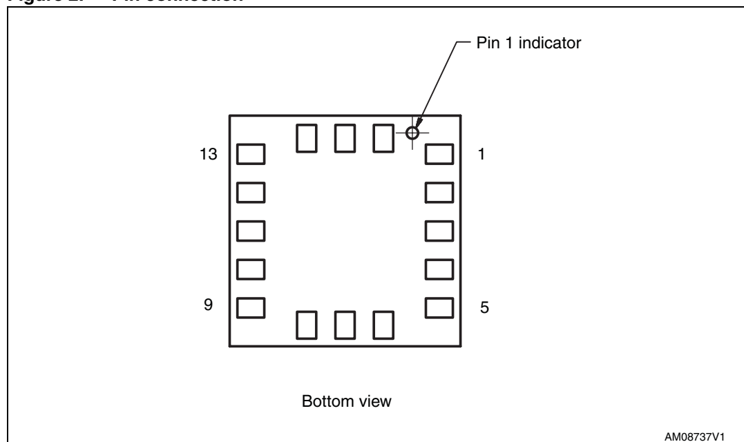
Figure 2. Pin connection
